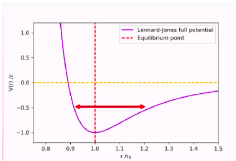
Figure 7.2: LJ Potential
